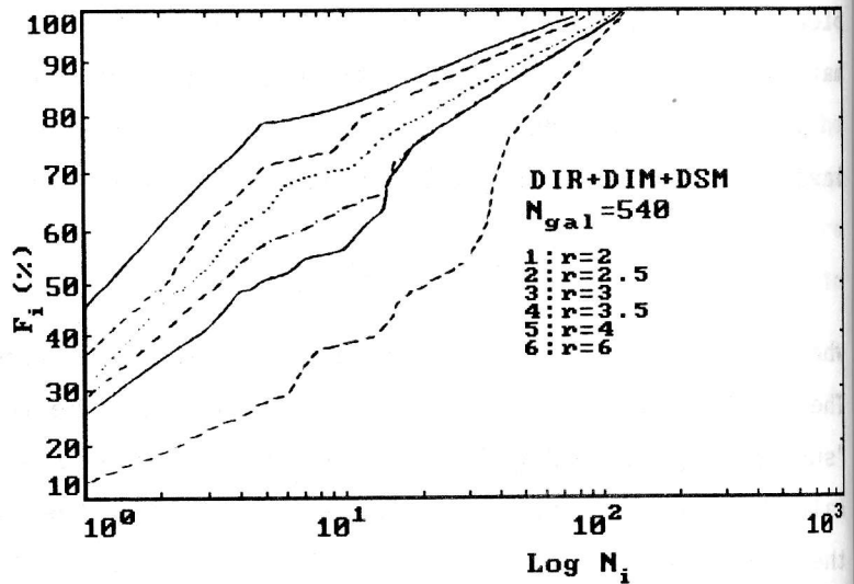
Fig.2. Clustering of dIr+dIm+dSm dwarfs (the whole Catalogue).
