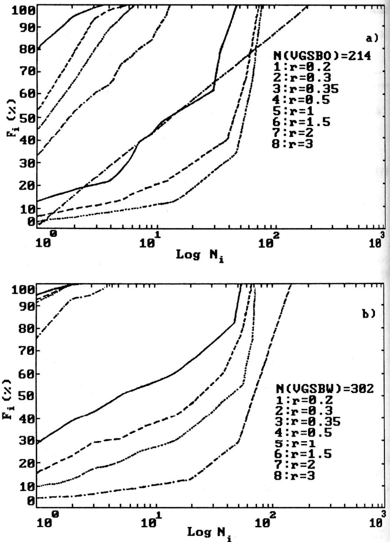
Clustering of dwarfs without nucleus and with implied nucleus as dependent on r (the Virgo cluster)
