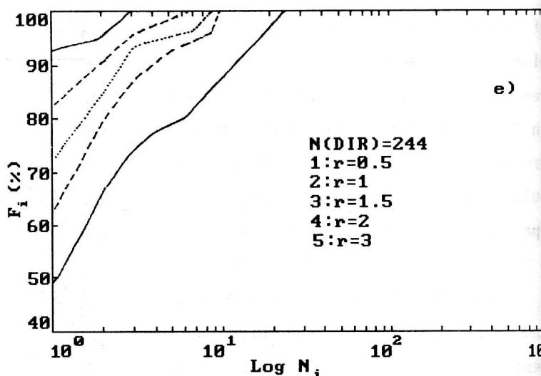
Fig.4. Clustering of dwarfs of the Catalogue divided into subsamples by types: a) dE, b) dSph, c) dSm, d) dIm, e) dIr (the whole Catalogue).
