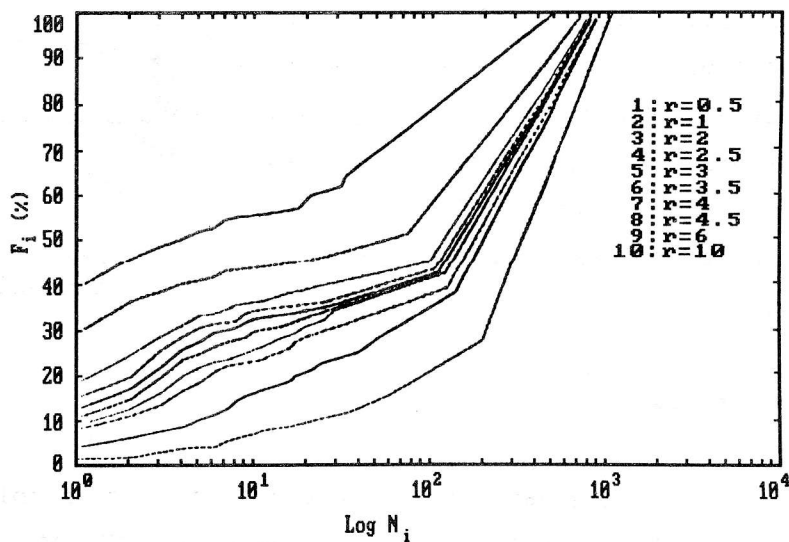
Fig. 1. Clustering of all LSB dwarfs of the Catalogue for a set of clustering radii. The abscissa is the logarithm of the number of dwarfs in a cluster ( \log N_i ), the ordinate is the integral fraction of galaxies entering clusters with a population N_g < N_i , F_i (%). The upper curve corresponds to the minimum clustering radius. The clustering radii are expressed in angular degrees. The designations in all the following figures are the same as in Fig. 1
