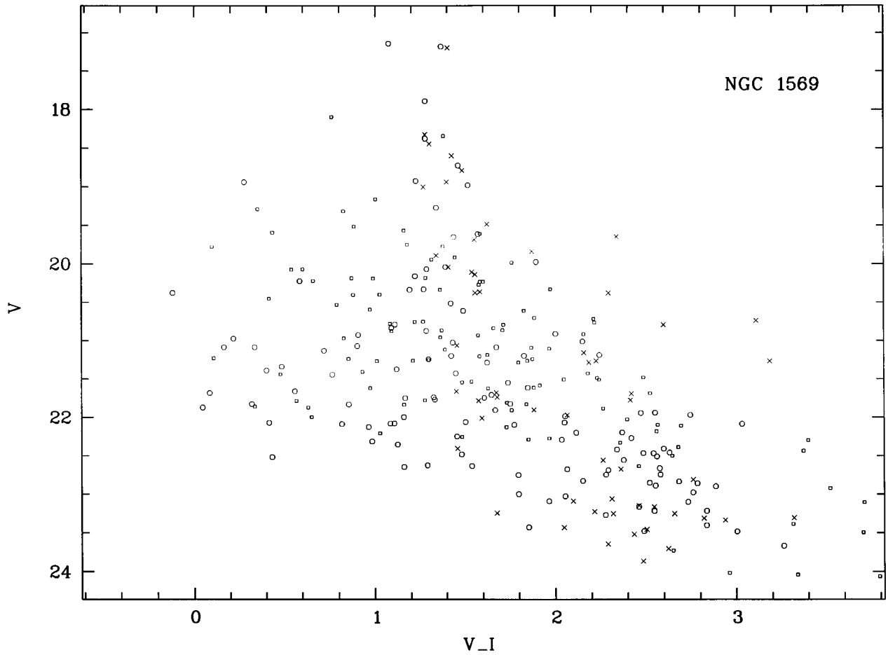
Fig. 9. V vs. (V - I) diagram for NGC 1569. Open circles correspond to stars measured in the main body of the galaxy, crosses indicate foreground stars, open squares represent the stars in the central region of the galaxy measured with the Hubble Space Telescope by O’Connell et al. (1994)
