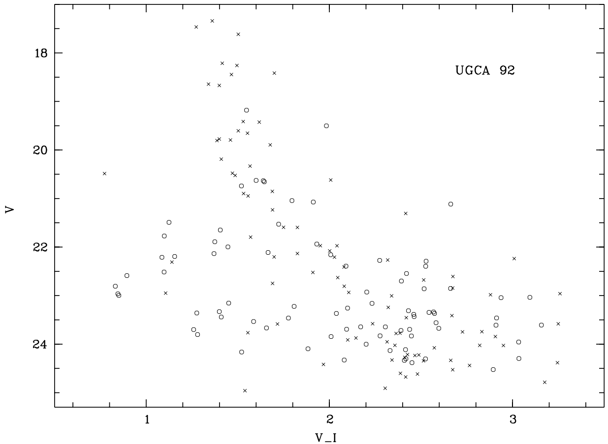
Fig. 5. Colour–Magnitude diagram for UGCA 92. the stars inside and outside the galaxy body are indicated by open circles and crosses, respectively
