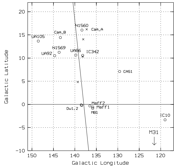
Fig. 1. The distribution of galaxies in the IC 342/Maffei complex in galactic coordinates. The open circles represent galaxies with radial velocities V_0 < 500 km/s, the crosses correspond to other probable members of the complex. The inclined solid line is the Supergalactic equator
