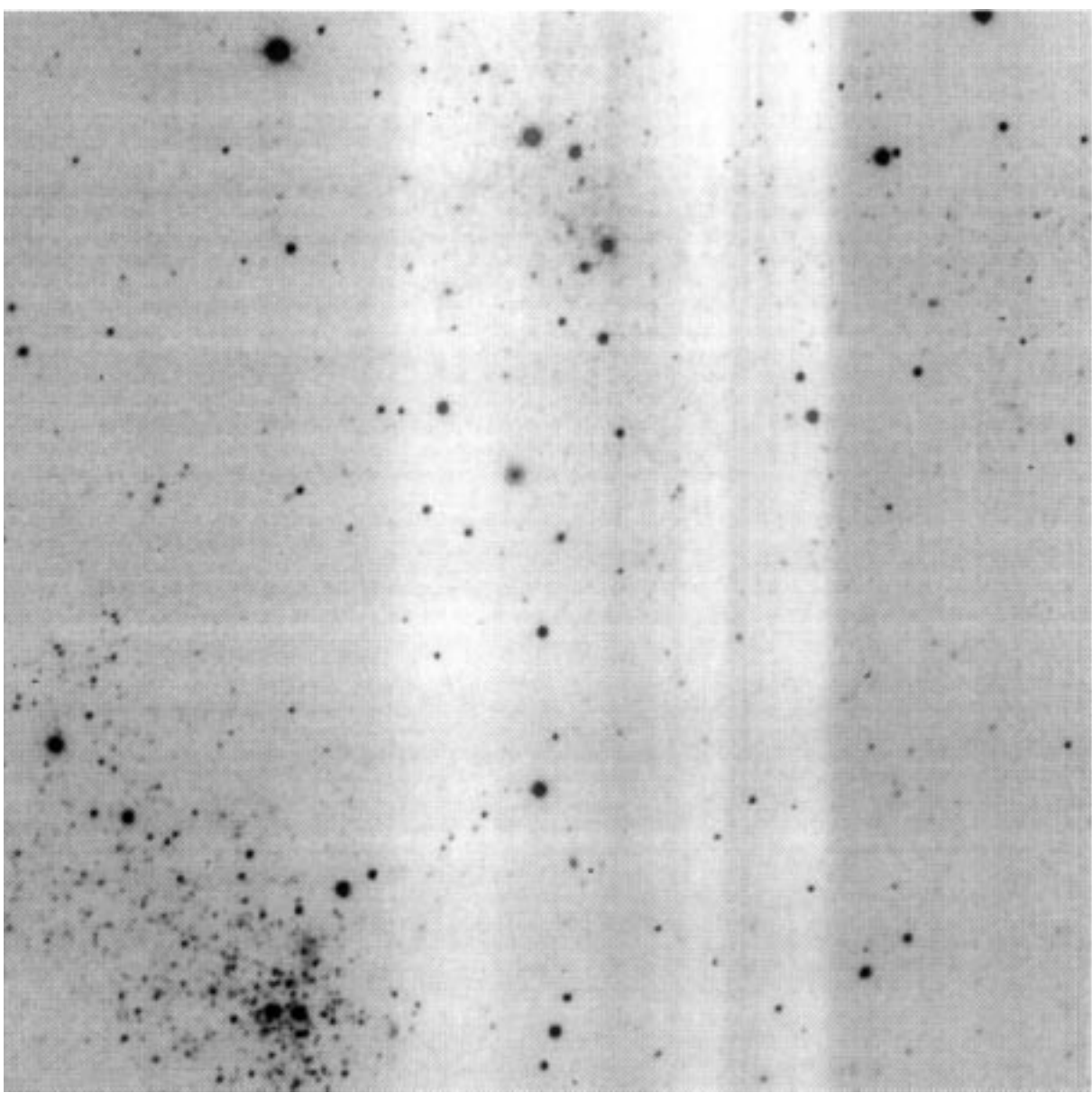
Fig. 6. The central part of UGCA 86 (above) and the bright southern superassociation (the lower left corner) in the I band
