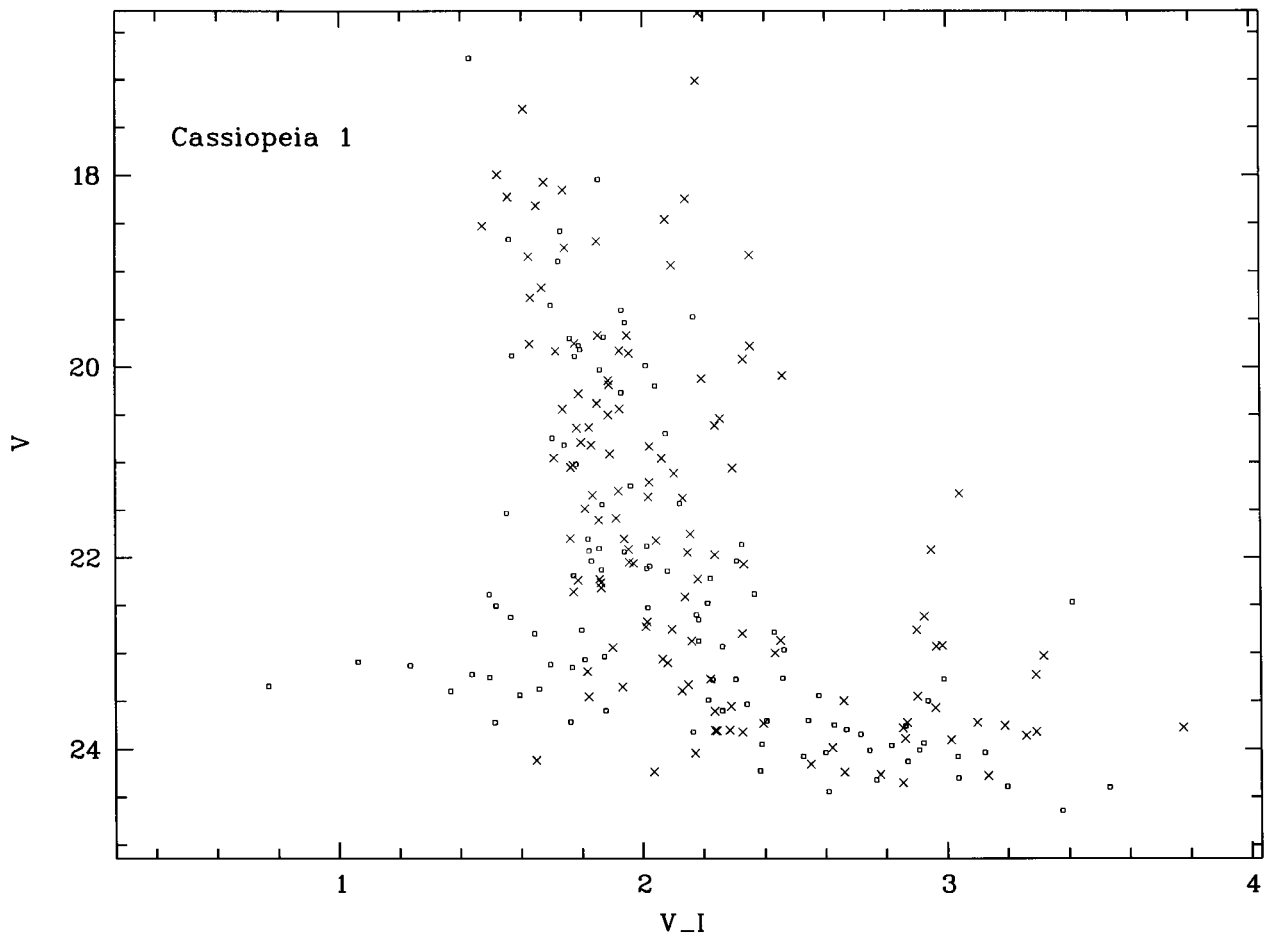
Fig. 11. V vs. (V - I) diagram for Cas 1. Stars within the galaxy body are indicated by open squares the remainder of the frame stars are noted by crosses
