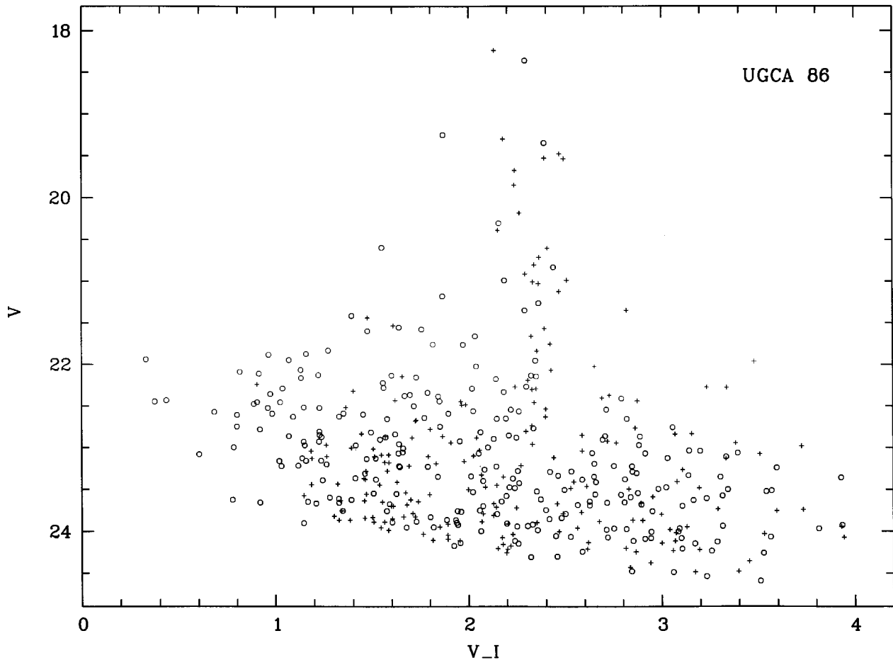
Fig. 7. Colour-Magnitude diagram for the southern concentration (open circles) and for the rest of the field of UGCA 86 (crosses)
