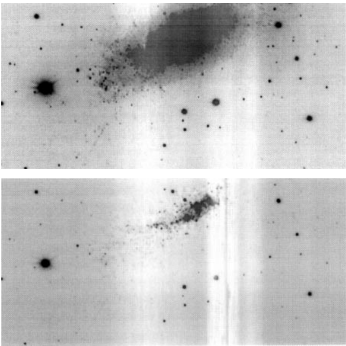
Fig. 8. NGC 1569 in the I band. a) Southern half of the original frame, b) the same part after subtracting the frame smoothed with a window of 10 \times (FWHM)
