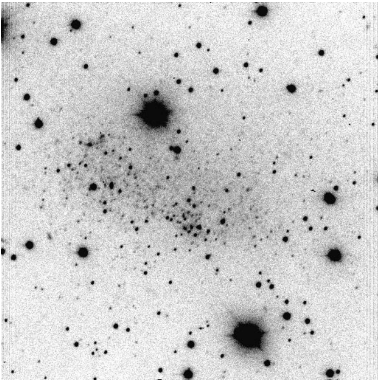
Fig. 4. UGCA 92 in the I band. The size and the orientation of the frame are the same as previously
