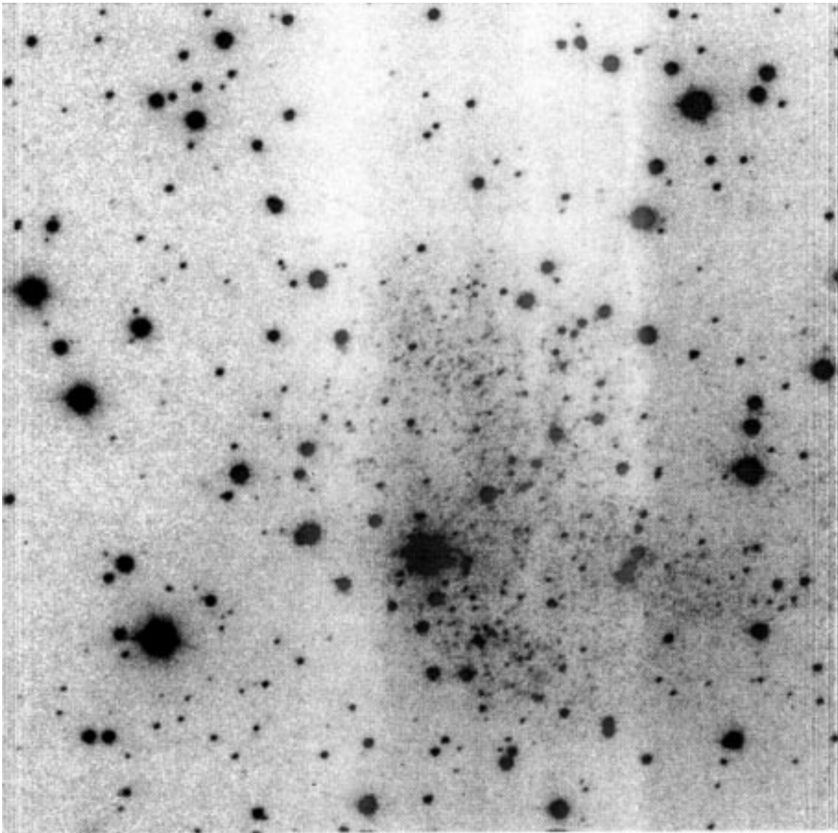
Fig. 10. CCD image of Cassiopeia 1 in the I band
