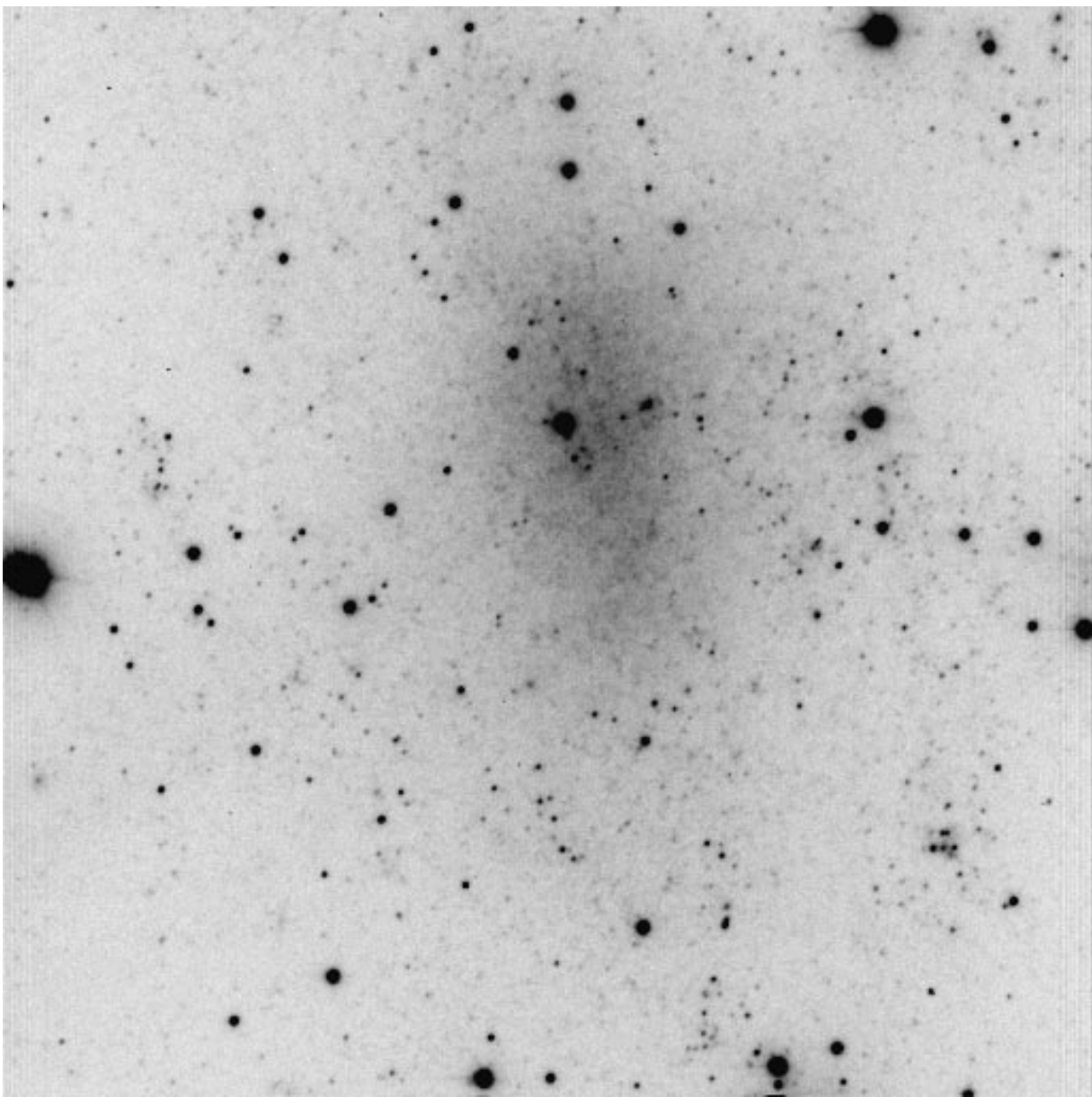
Fig. 2. The central part of UGCA 105 in the I band. The size of the CCD frame is 3.0 by 3.0 arcmin. North at top, East on the left
