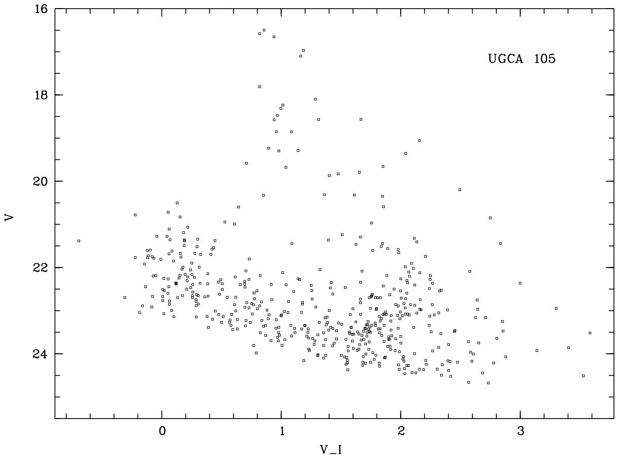
Fig. 3. Colour–Magnitude diagram for 568 stars in UGCA 105
